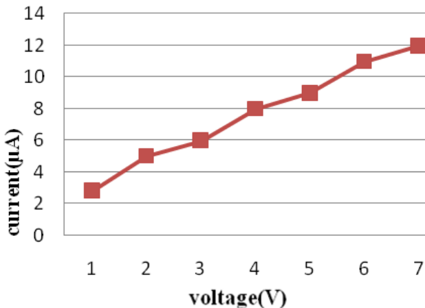
Fig 4: V-I graph of parallel and series connection
