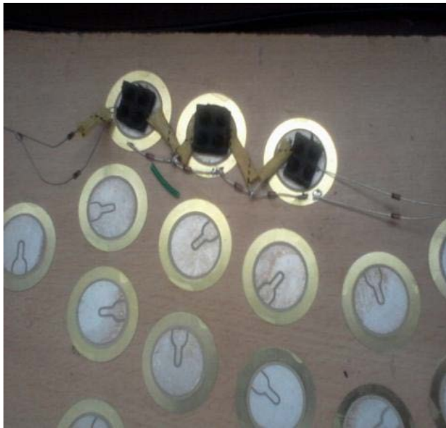
Fig 3: PZT in series connection
