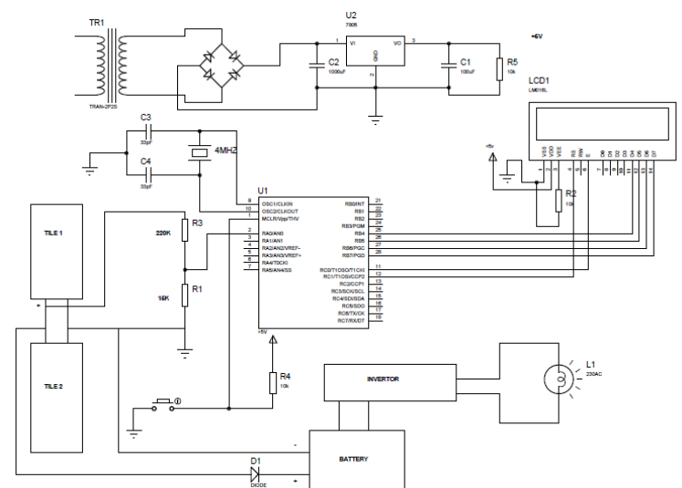
Fig 6: Hardware setup
