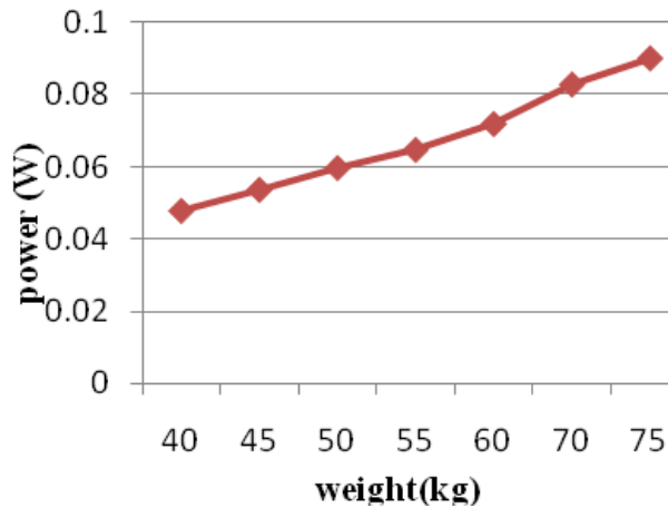
Fig 8: Weight V/s power graph of piezo tile
