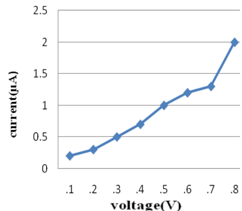
Fig 2: V-I graph of PZT
